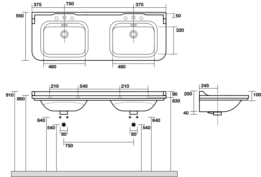
4143 Lavabo150x55 doppia vasca sospeso monoforo (tre fori a richiesta) One hole wall hung double basin 150x55 (three holes on demand)
