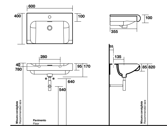
3411 “INKA” lavabo semincasso 60x40x35,5 monoforo “INKA” one hole semi recessed washbasin 60x40x35,5
