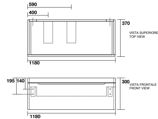
911101 “INKA” mobile sospeso 120 cm versione lavabo sinistro “INKA” wall mounted cabinet 120 left hand basin 911102 “INKA” mobile sospeso 120 cm versione lavabo centrale “INKA” wall mounted cabinet 120 central basin
