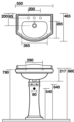
1045 Lavabo 55 monoforo (tre fori a richiesta) One hole washbasin 55 (three holes on demand) 1070 Colonna Pedestal
