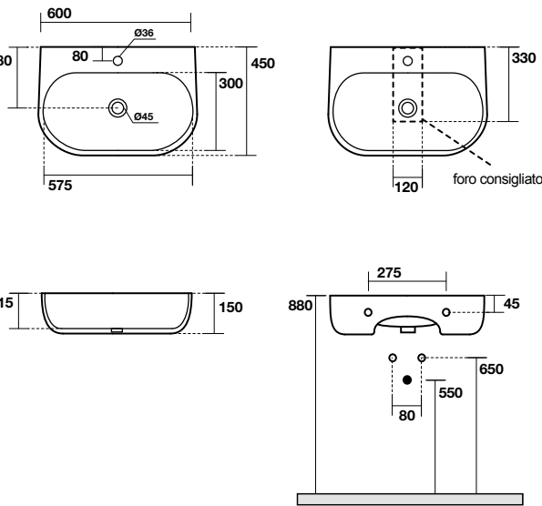
5343 Lavabo ovale appoggio cm 60 oval counter top washbasin cm 60
