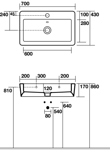
4302 Lavabo ciotola C2 appoggio Ø 46 H 17 Free standing washbasin ciotola C5 Ø 46 H 17
