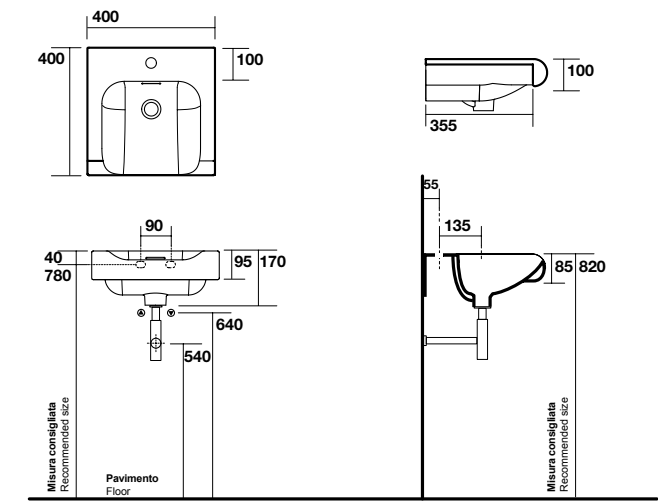
INKA Piano in ceramica -- INKA Ceramic counter
