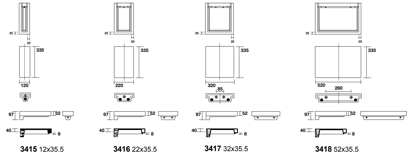
INKA Piano in ceramica -- INKA Ceramic counter
