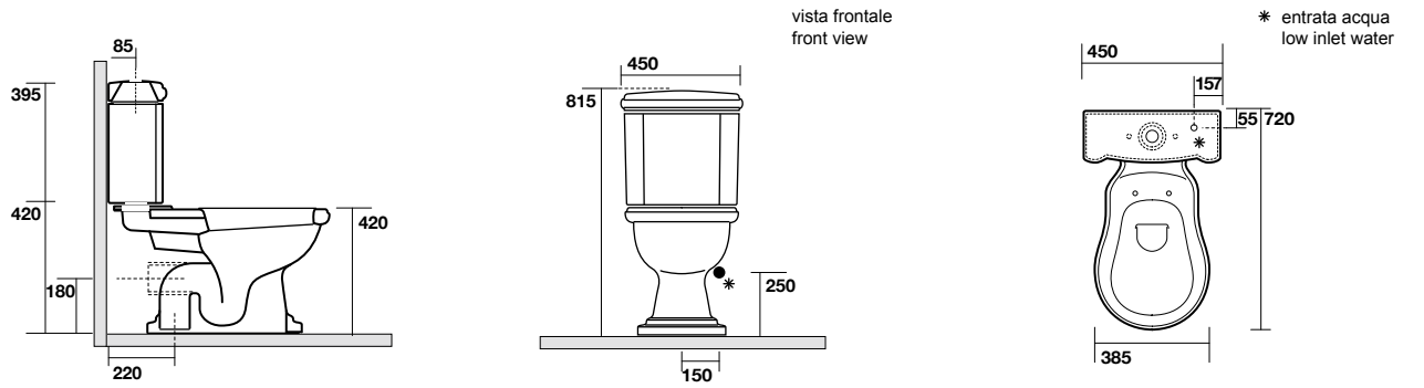
1081 Cassetta monoblocco Close coupled cistern
